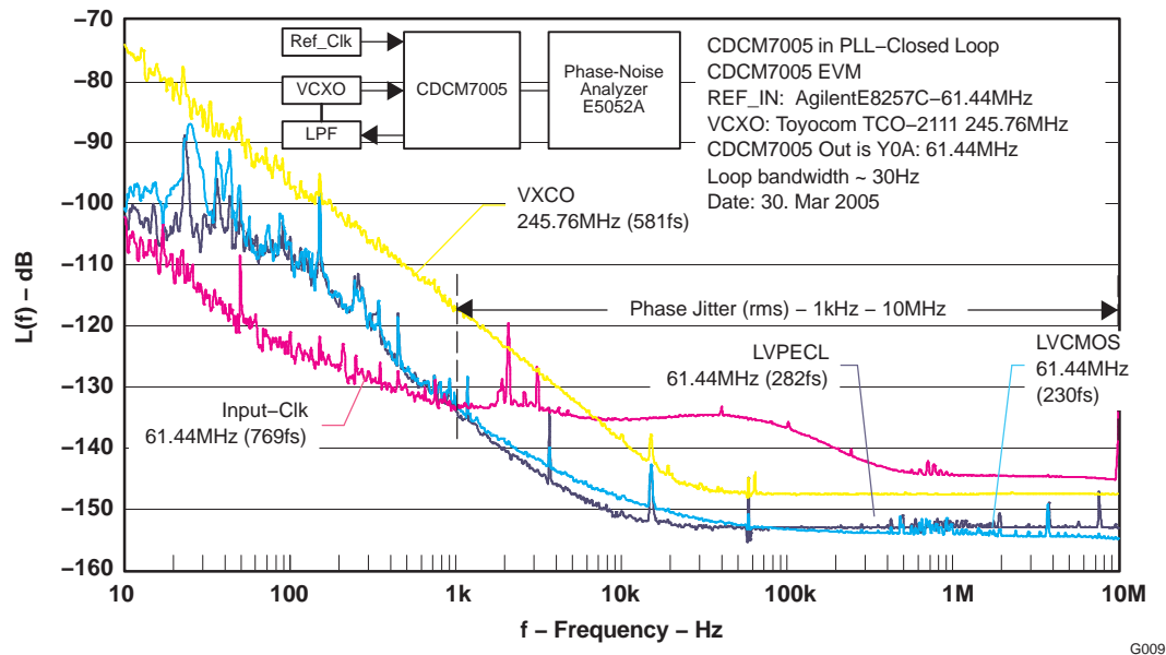
Figure 28. Phase Noise (61.44-MHz REF_IN and 61.44-MHz Output Frequency)
