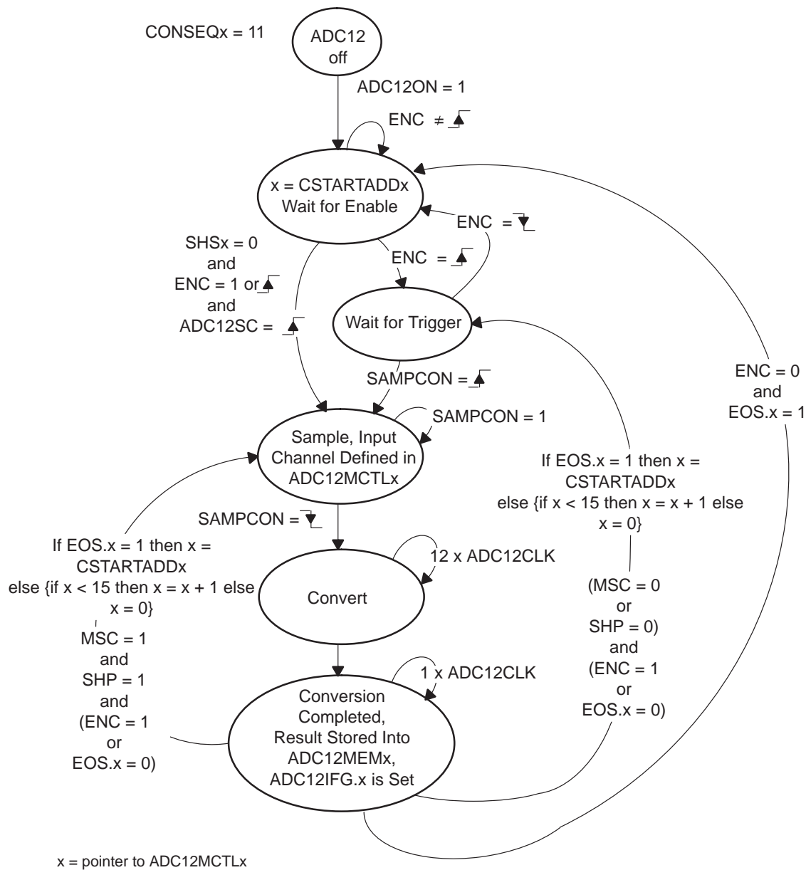
Figure 17–9. Repeat-Sequence-of-Channels Mode
