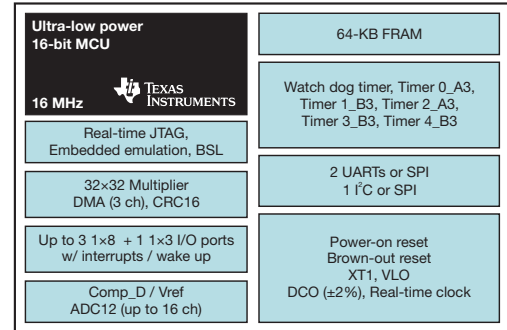
MSP430FR5969-SP
