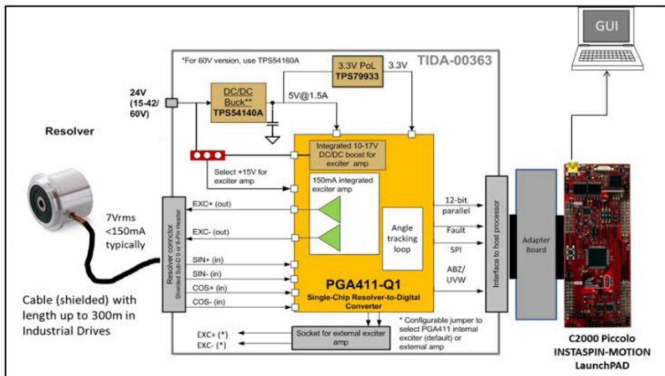
Figure 1. Simplified System Block Diagram of the TIDA-00363 Reference Design with F28069M MCU LaunchPad™ Development Kit
