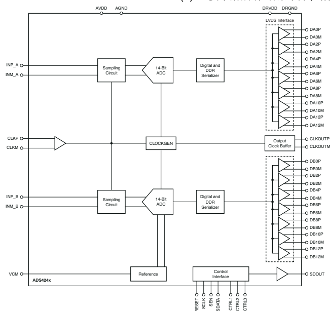
ADS4222/25/26/42/45/46 方框图
