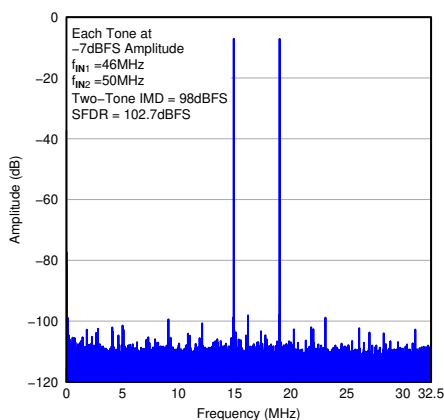
图 7-52. FFT for Two-Tone Input Signal
