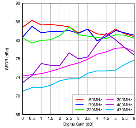
图 7-77. SFDR vs Gain and Input Frequency
