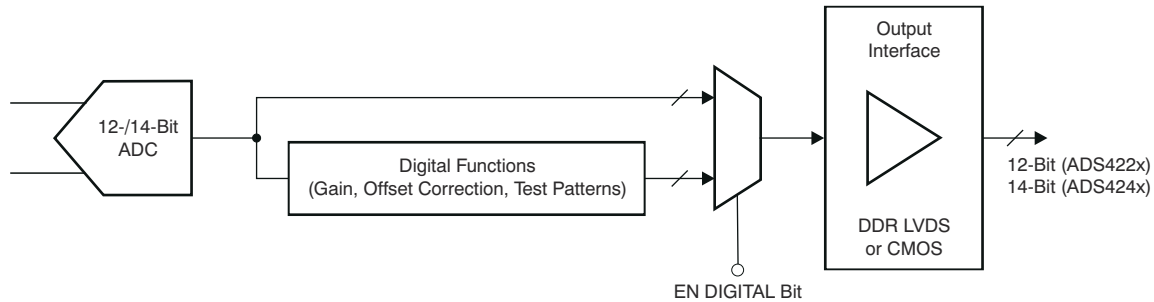
图 8-15. Digital Processing Block
