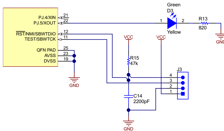
图 10. Programming Connector
