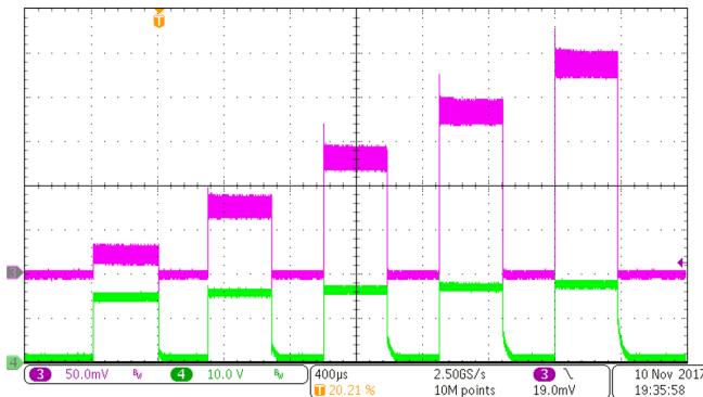
图 48. Current Bracketing: On Time = 400 μs, Frame Rate = 1428 Hz, N = 5, I LED = 200 mA, Current Brk = 550 mA, 5 Steps From 200 mA to 2.4 A in 4 Increments of 550 mA
