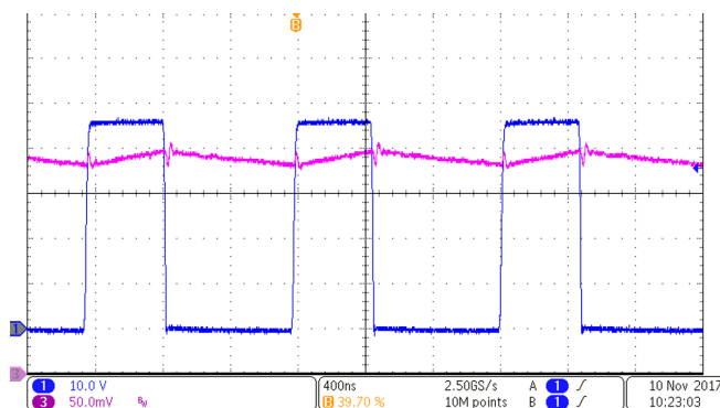
图 57. Buck Switch Node at 2400 mA of LED Current
