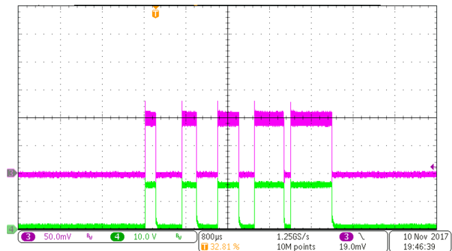
图 49. Time Bracketing: On Time = 400 μs, Frame Rate = 1428 Hz, N = 5, I LED = 1000 mA, Time Brk = 0.5
