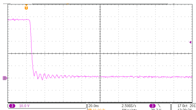
图 63. Pre-Boost Switch Node, Falling, R34 = 0 \Omega , R35 = 3.32 \Omega
