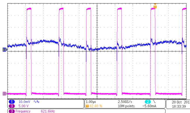
图 69. 5-V Buck: SW and VOUT Ripple; 36-V Input
