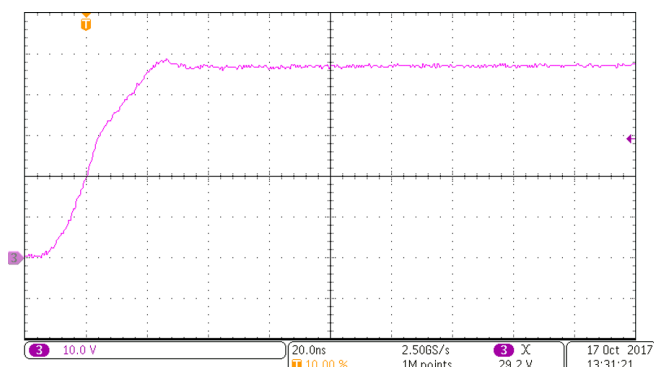
图 62. Pre-Boost Switch Node, Rising, R34 = 0 \Omega , R35 = 3.32 \Omega
