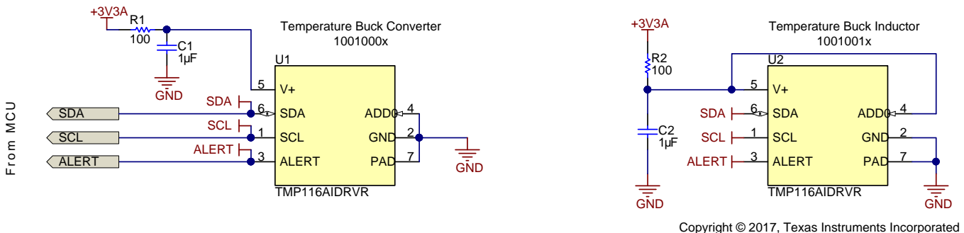
图 31. Temperature Sensors of LED Buck
