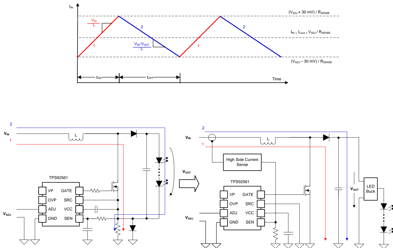
图 33. Pre-Boost Operation—Standard vs Modified Implementation and Input Current Waveform
