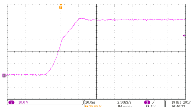
图 64. Pre-Boost Switch Node, Rising, R34 = 15 \Omega , R35 = 15 \Omega
