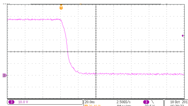
图 65. Pre-Boost Switch Node, Falling, R34 = 15 \Omega , R35 = 15 \Omega
