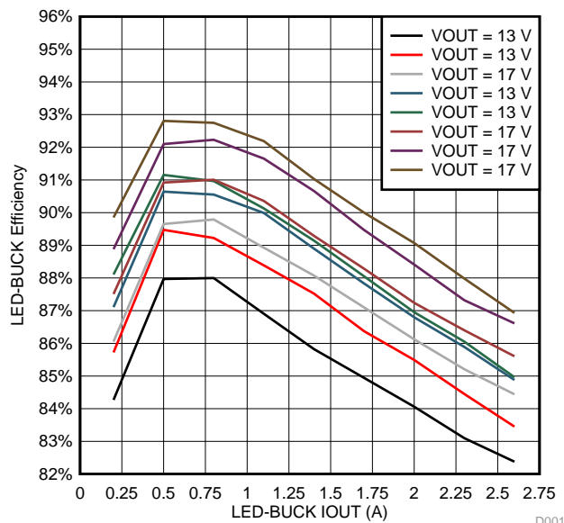
图 54. Efficiency vs IOUT
