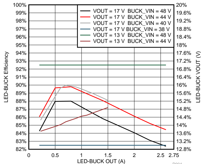
图 55. LED Efficiency and VOUT vs IOUT: Comparing Test With LED Board vs Resistive Load
